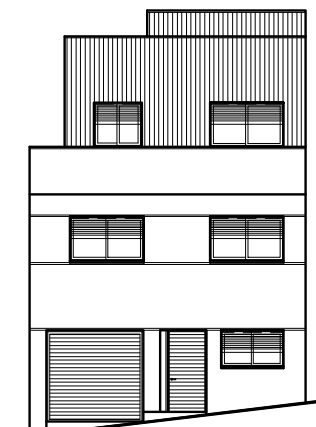
ALZADO PRINCIPAL
